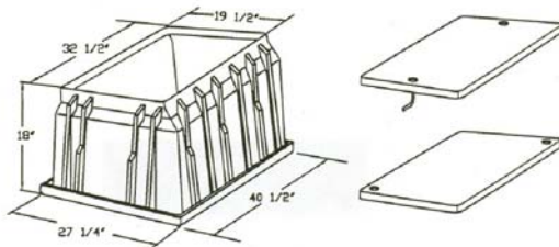
CARSON IND. SERIES 1730D BOX W/COVER (OR EQUIVALENT) USED FOR ALL ASSEMBLIES 2" AND SMALLER
