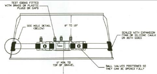
DOUBLECHECK ASSEMBLY DETAIL
